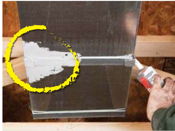
Seal ducts at joints to prevent heated or cooled air from leaking out or unconditioned air from leaking into the ducts.
